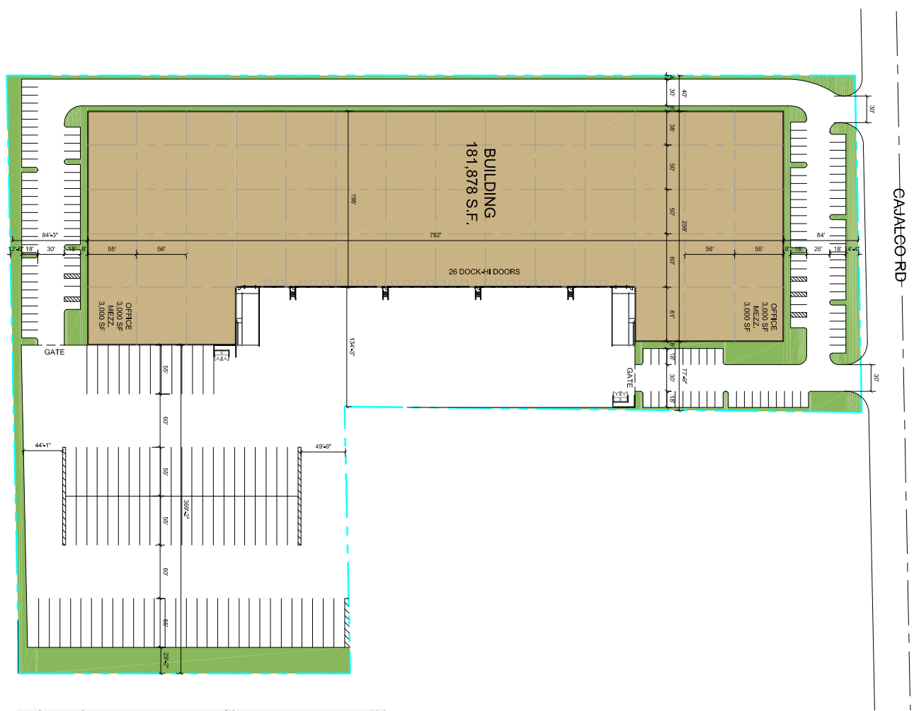
A CONCEPTUAL SITE PLAN SCALE: 1" = 40'
